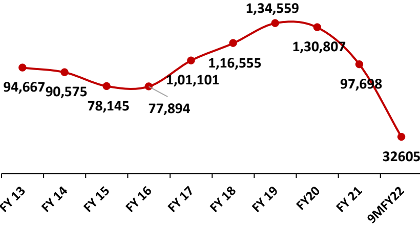
HB Wire Production (mt)
